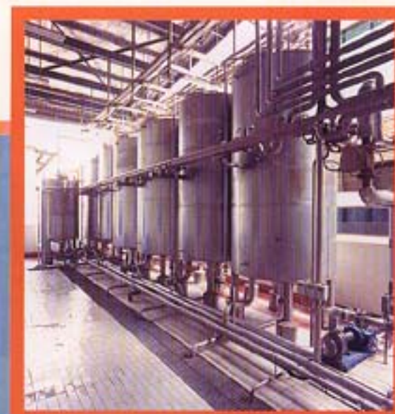
CIP PLANT
