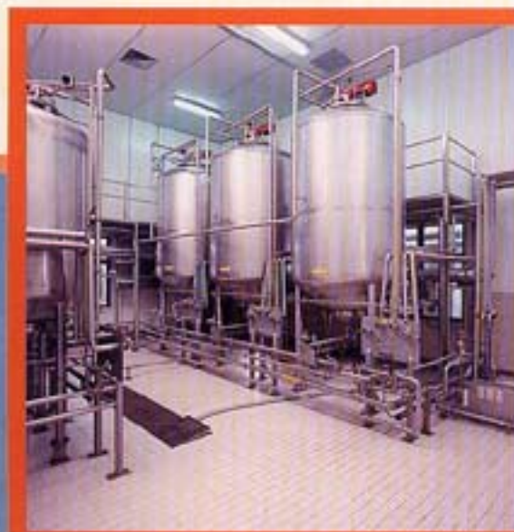
YEAST PITCHING VESSELS
